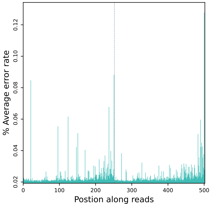
Error rate distribution along reads (R20123)
